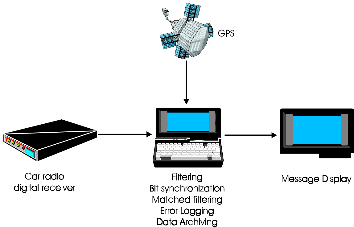
Figure 4. Herald Data Reception Flow Chart
