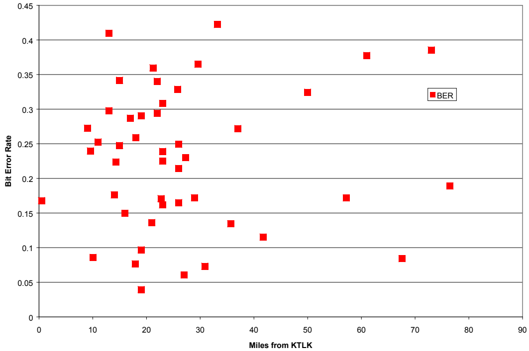
Figure 13. Bit Error Rate By Distance from KTLK
