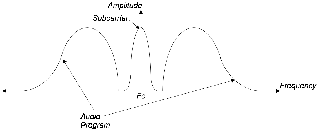
Figure 2. Herald subcarrier data placement on AM channel
