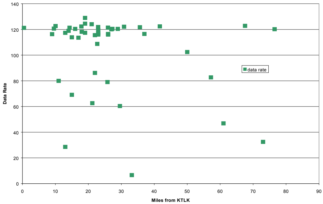
Figure 11. Herald Data Rate by Distance from KTLK
