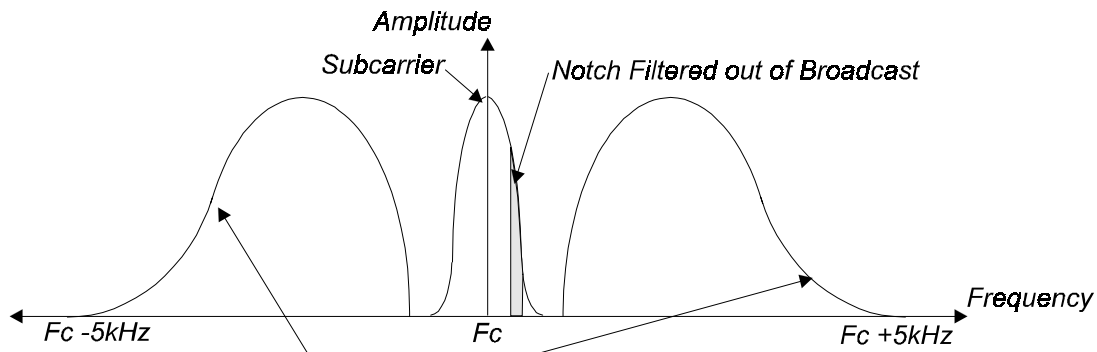
Audio Program Figure 17. A notch filter in the AM subcarrier
