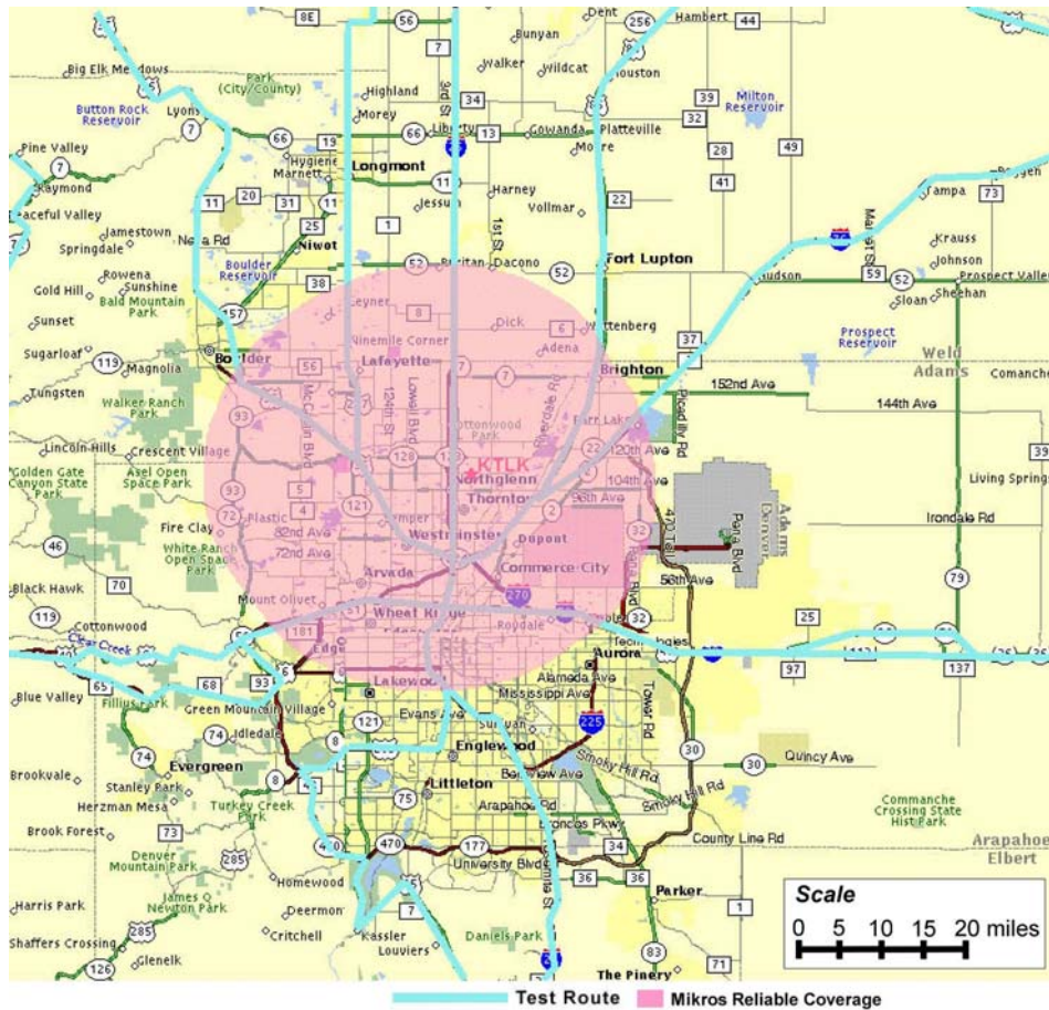
Figure 16. Mikros System Coverage
