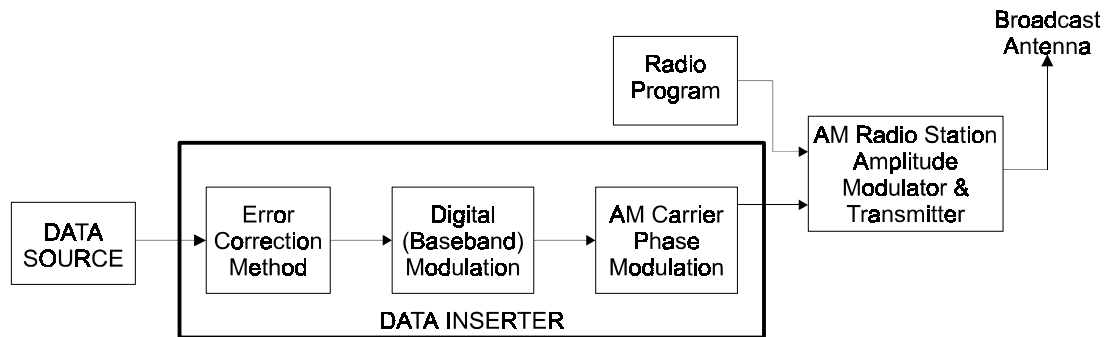
Figure 5. Mikros system data creation and transmission
