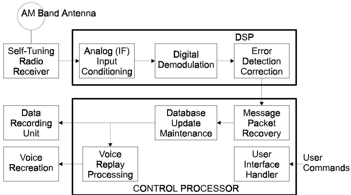
Figure 6. Mikros system data receiver
