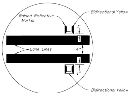
Figure 10 FDOT Standard Index Guidance for Placement of Raised Pavement Markers
