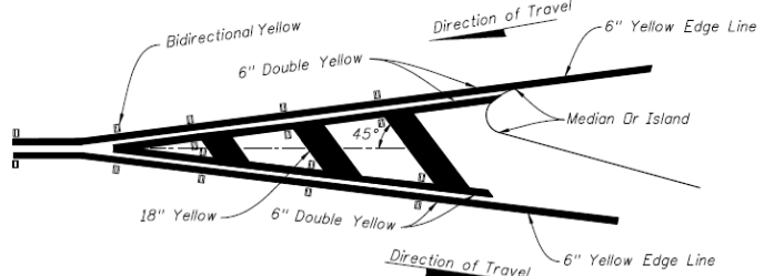
RPM PLACEMENT FOR TRAFFIC SEPARATION (TRAFFIC FLOWS IN OPPOSITE DIRECTION)
