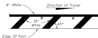
PLACEMENT OF RPM'S ON SHOULDER MARKINGS
