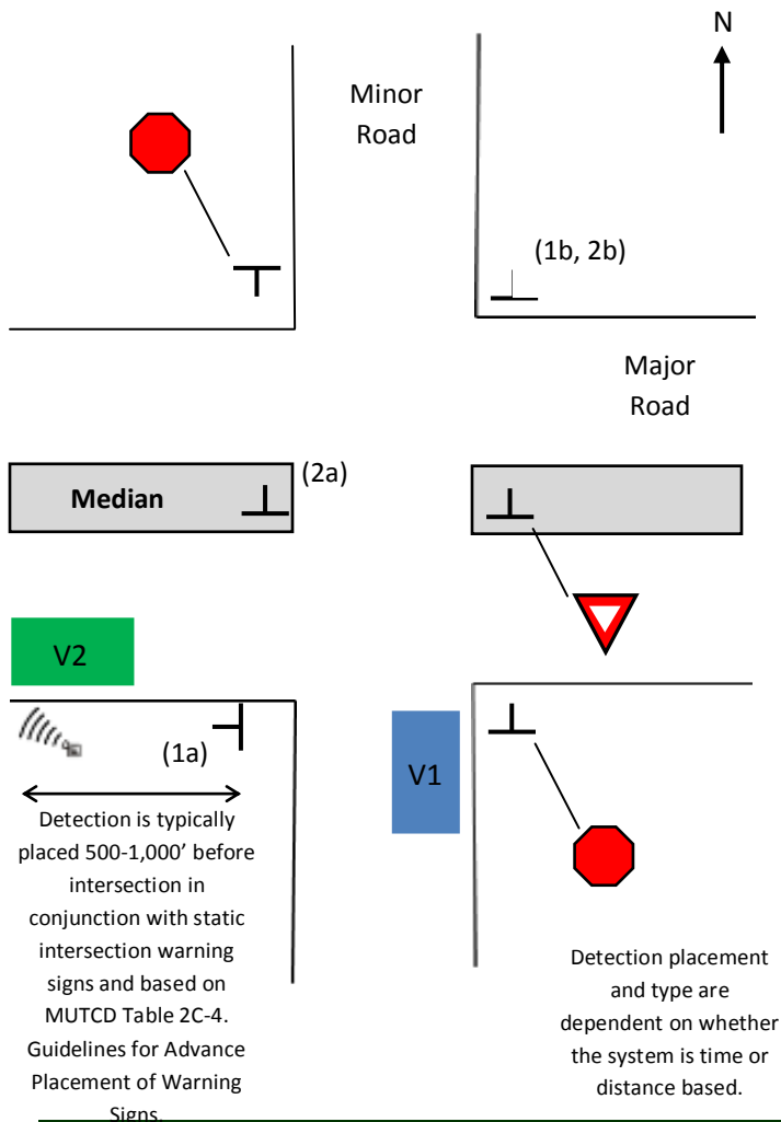
Figure 3 Minor Road Alert for 2-Lane/Multi-Lane Median Separated Intersection
