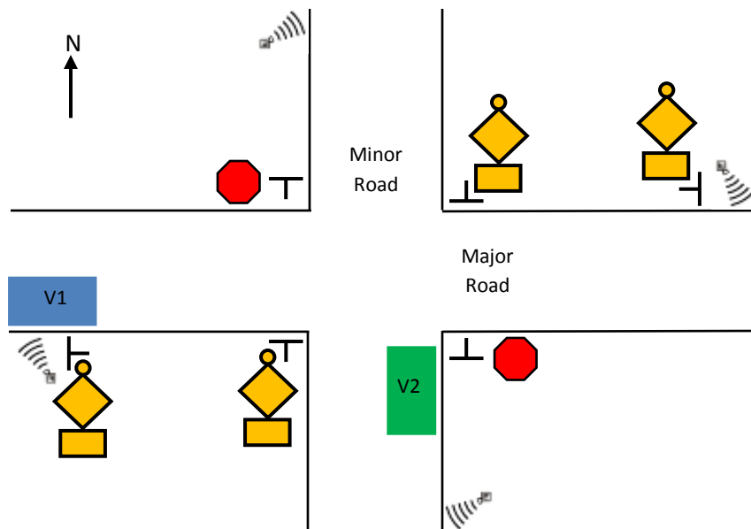
Figure 1 Typical Intersection Conflict Warning System Concept
