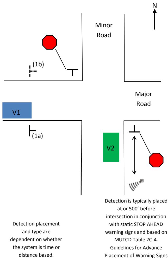
Figure 4 Major Road Alert for 2-Lane/2-Lane (or Multi-Lane) Intersection
