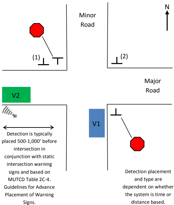
Figure 2 Minor Road Alert for 2-Lane/2-Lane (or Multi-Lane) Intersection
